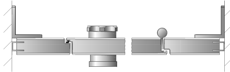
2 Sectional view: front wall with one hand door knob Rising hinges made of aluminium
