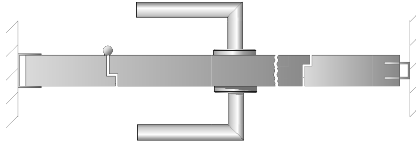
2 Cubicle front section with door handle. Optional wall connection with U-profile as a shadow gap
